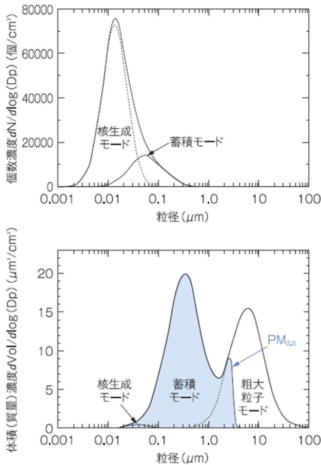
図2 都市大気粒子の粒径分布 (出典：William C. Hinds, 1999, Aerosol Technology, A Wiley-Interscience Publication を和訳と追記)
